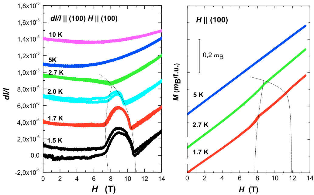
Figure 1: Field dependency of the isothermal longitudinal forced magnetostriction (left) and of the magnetization (right) of single-crystalline \text{CeCu}_2\text{Ge}_2 for magnetic fields parallel to the crystallographic [100] axis. Phase transitions are indicated by dotted lines.
